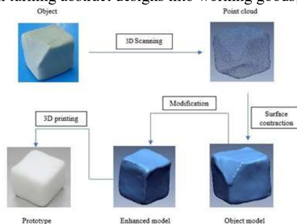
FIG.1. Conventionalreverseengineering[3]
